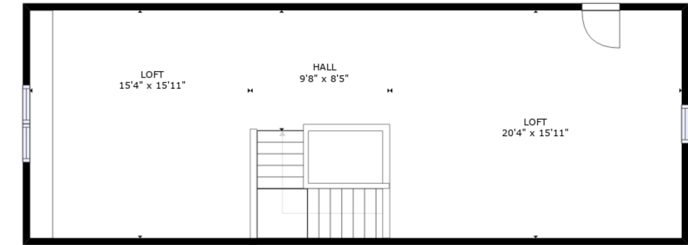
FLOOR 3
